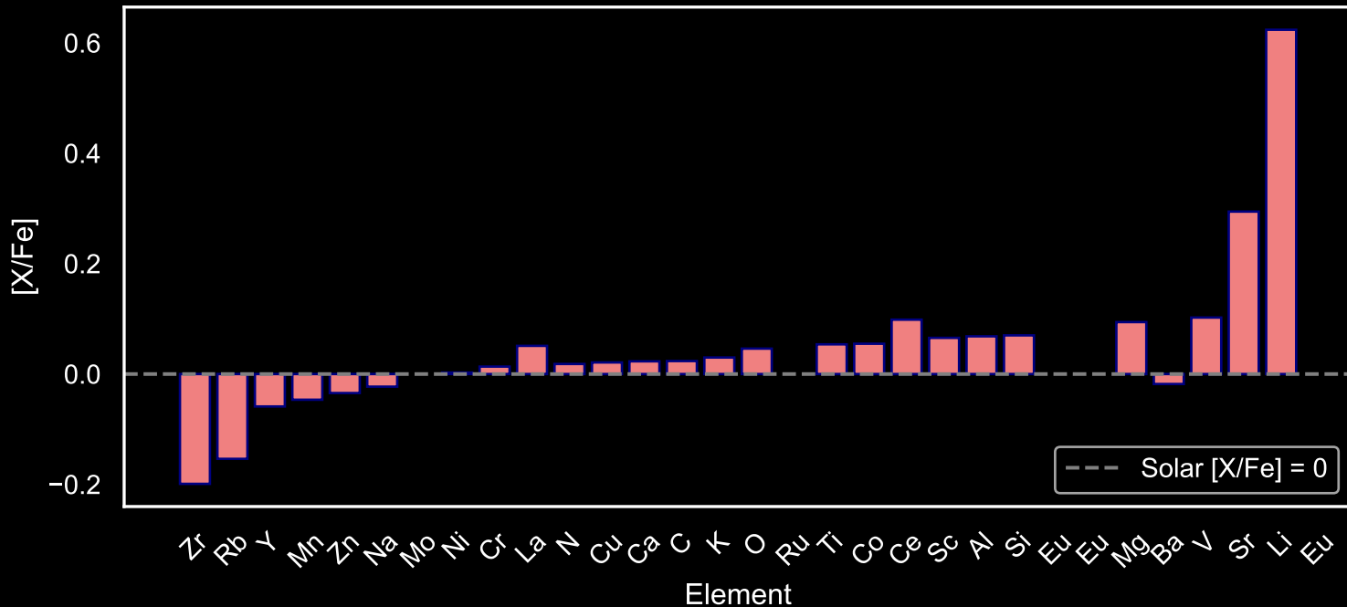
Abundance Pattern for GALAH Main Sequence Stars: Star Field [92] (N=95)
