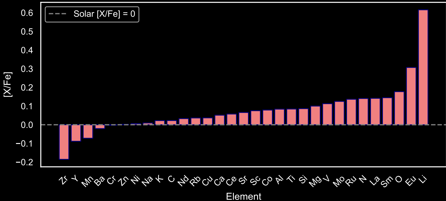
Abundance Pattern for GALAH Star Field [92] (N=224)
