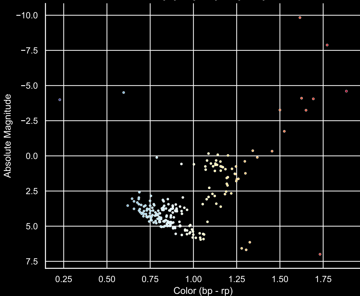
GALAH Hertzsprung-Russel Diagram Field [92] Ra [16.22] Dec [-73.66]
